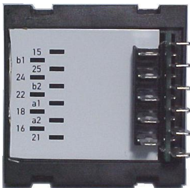
Rear view: terminal block
